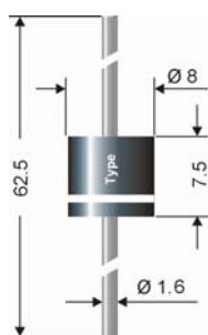
Axial Lead Diode
