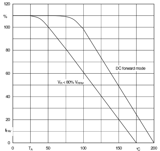
Fig. 2: Rated forward current vs. ambient temperature 1)
