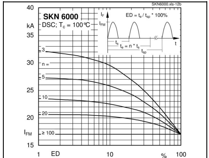
Fig. 10b Peak forward current vs. duty cycle ( T_c = 100\text{ °C} )
