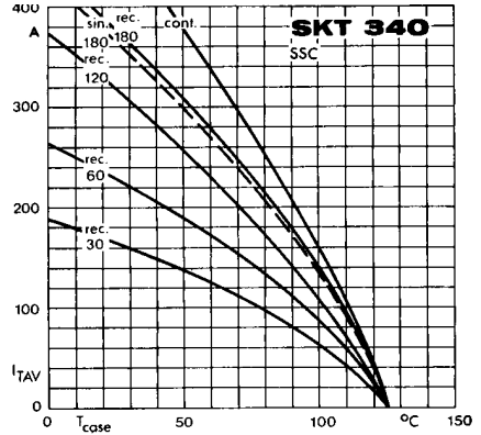
Fig. 2 d Rated on-state current vs. case temperature
